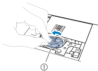
① SpulenkapSEL
